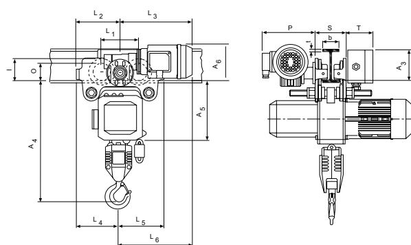
CPEF 1 /CPEF with integrated electric trolley
