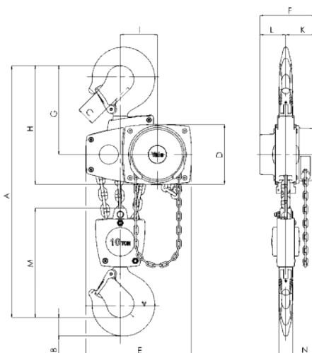
Yalelift 360, 10000 kg, three falls
