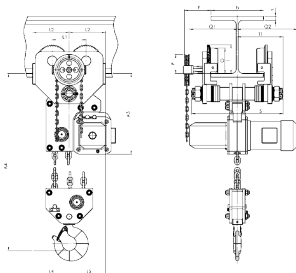
CPEF 1 /CPEF with integrated geared or electric trolley, 7500 kg
