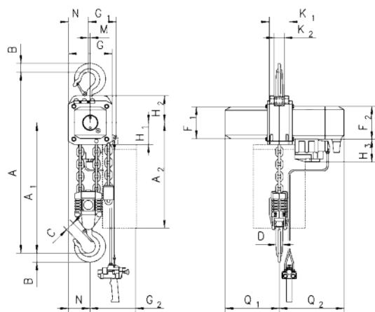
CPA with suspension hook, 4000 - 5000 kg, double fall
