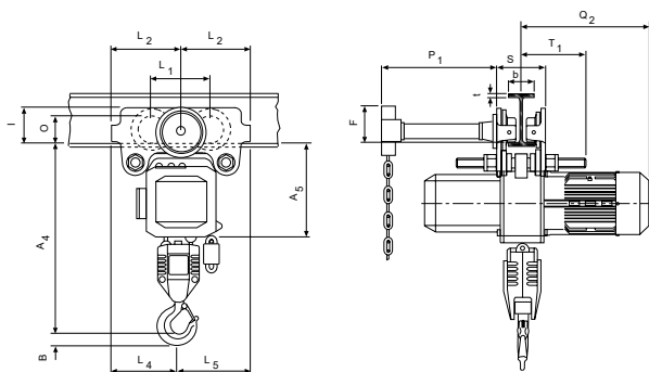
CPEF 1 /CPEF with integrated manual geared trolley
