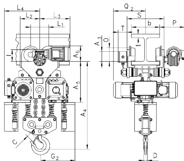
CPEF 1 /CPEF with integrated electric trolley, 10000 kg
