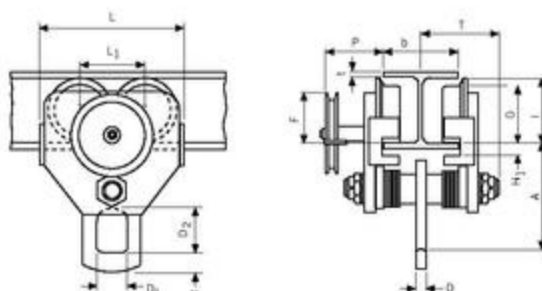
Model HTG 10000 kg
