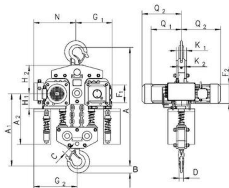
Model CPE/CPEF 100-2 with suspension hook, 10000 kg
