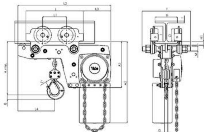
Model Yalelift LHP, 500 - 3000kg, single fall
