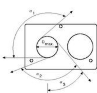
Rope lead-offs for electric winch RPE
