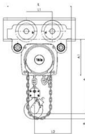
Model Yalelift ITG, 500 - 3000 kg, single fall
