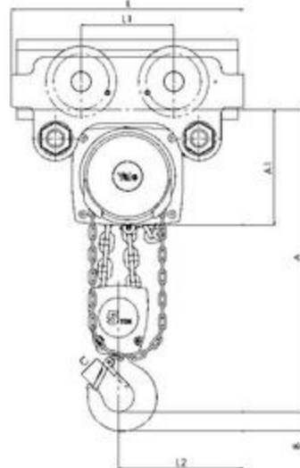
Model Yalelift ITP/ITG, 5000 kg, double fall
