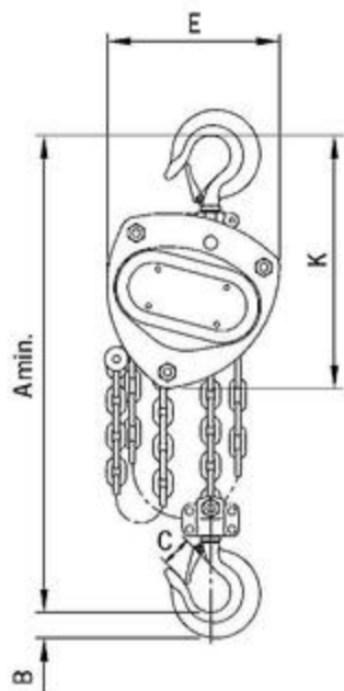
Model VSIII, 250 - 3000 kg, single fall
