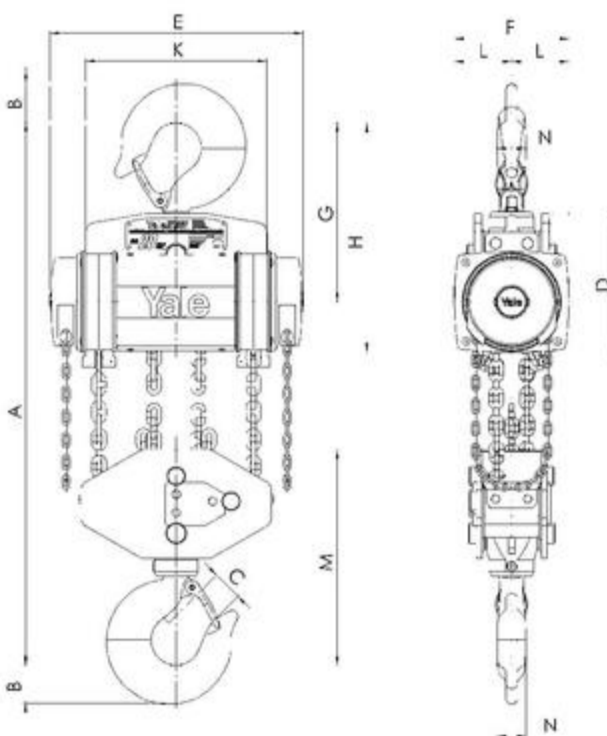
Model Yalelift 360, 20000kg, six fall
