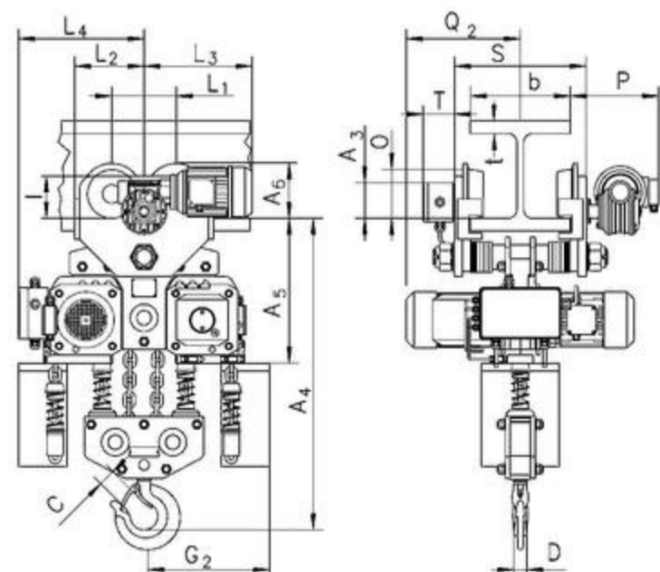
Model CPE/CPEF with integrated electric trolley, 10000 kg
