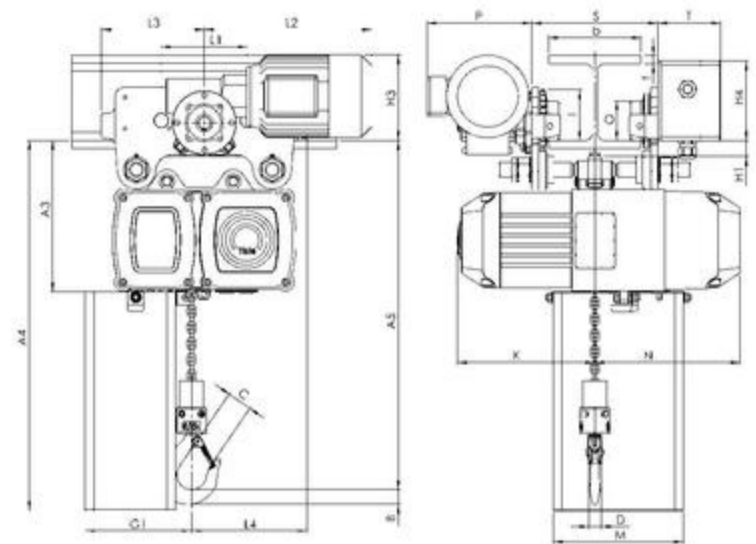
Model CPV/CPVF with integrated electric trolley
