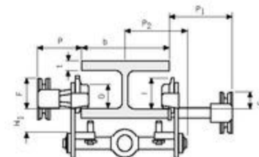
Model HTP/G 500 - 5000 kg, with locking device
