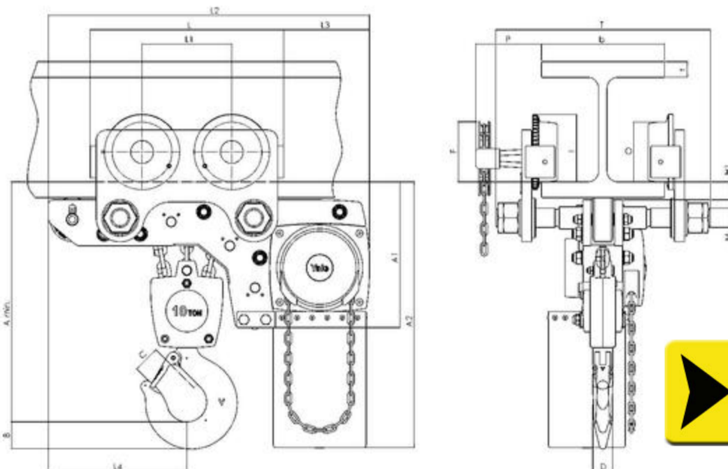
Model Yalelift LHG, 10000 kg, three fall
