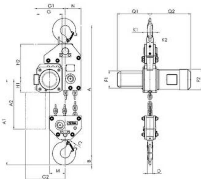
Model CPE/CPEF 75-1,6 with suspension hook, 7500 kg
