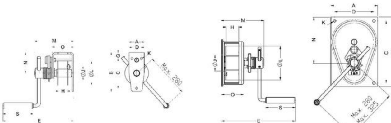
Model MWS, capacity 150 kg
