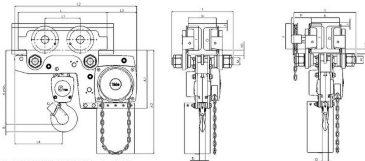
Model Yalelift LHP/LHG, 5000 kg, double fall
