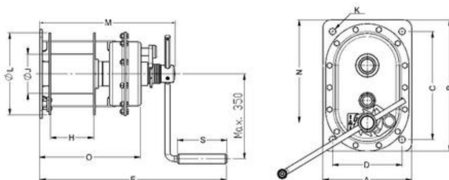
Model MWS, capacity 1000 - 1500 kg
