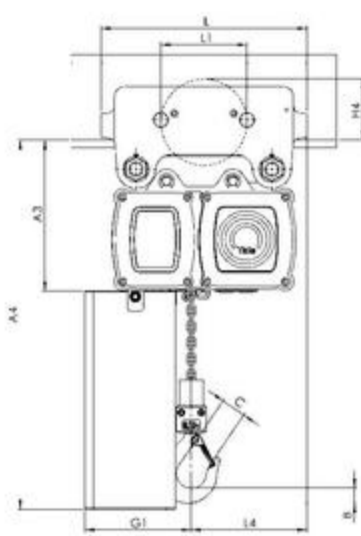
Model CPV/CPVF with integrated manual push or geared trolley
