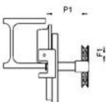
Model HTG 10000 kg, locking device
