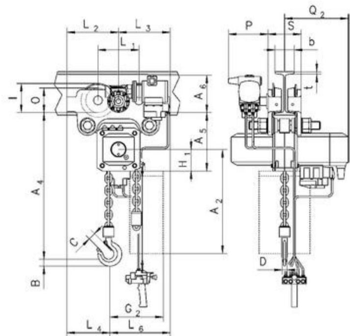
Model CPA with integrated pneumatic trolley
