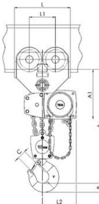
Model Yalelift ITG, 10000 kg, three fall
