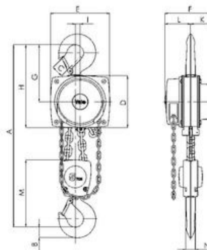
Model Yalelift 360, 5000kg, double fall
