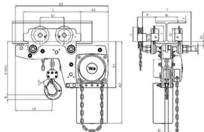
Model Yalelift LHG, 500 - 3000kg, single fall
