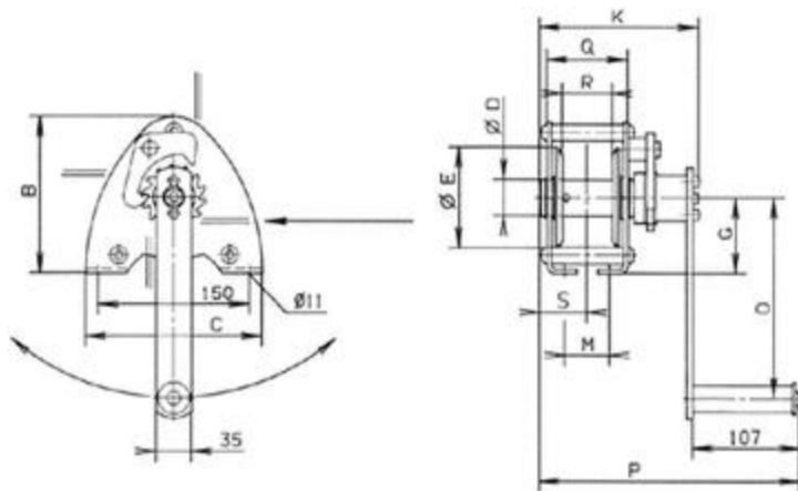
Model LB 150 - 350 kg
