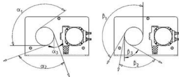
Rope lead-offs for pneumatic rope winch RPA
