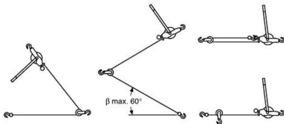
Rigging configurations - Attention! reduced capacity
