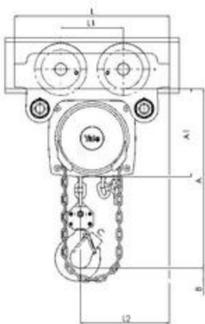
Model Yalelift ITP, 500 - 3000 kg, single fall
